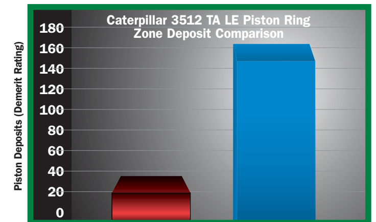
SENTRON LD 5000 is 860% cleaner than a leading competitive NGEO after 8000 hour field tests in the same Caterpillar 3512 TA LE engine. This can lead to significantly longer overhaul life using SENTRON LD 5000 in place of the leading competitor's NGEO.
