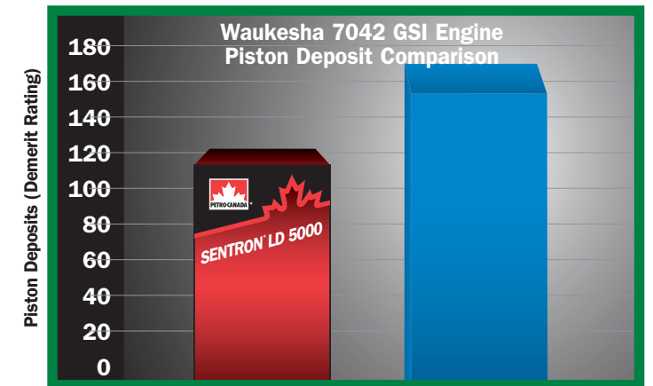
SENTRON LD 5000 has 25% less piston deposit than leading competitive NGEO in Waukesha 7042 GSI engines.
